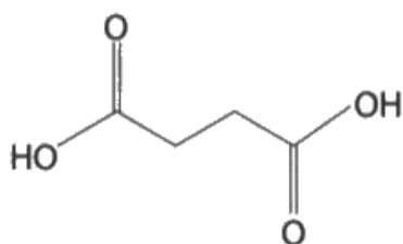
succinic acid
