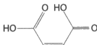
maleic acid
